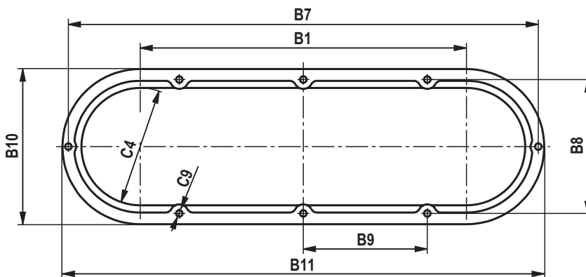
Hole pattern tank cover with installation plate
