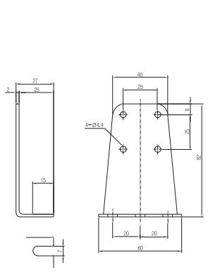
Mounting Accessory
